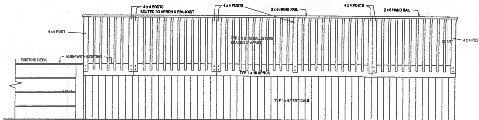
ELEVATION DETAIL
