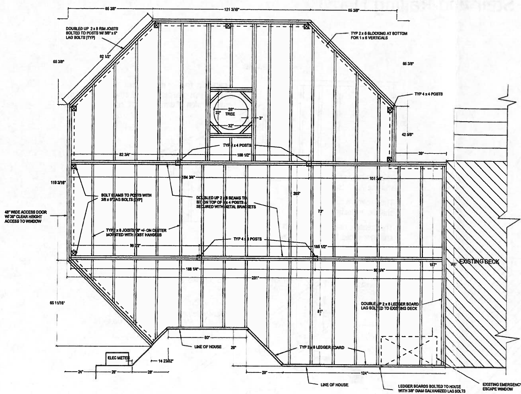
JOIST & POST PLAN LAYOUT
