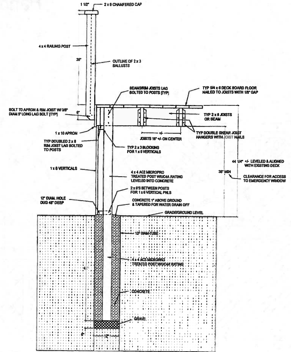
POST INSTALL W/ JOIST DETAIL
