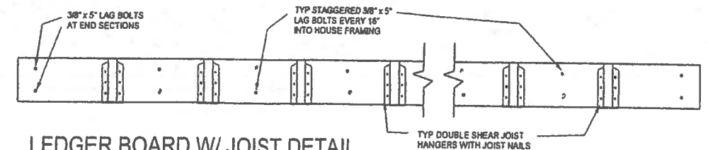
LEDGER BOARD W/ JOIST DETAIL
